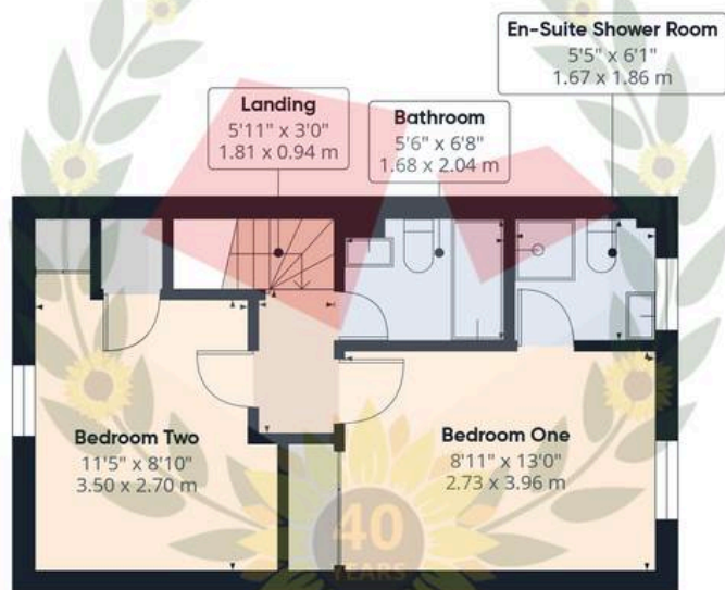
Floor 2 Building 1
